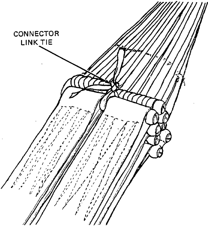
Figure 2-26. Risers and Connector Link Assemblies in Proper Arrangement.
