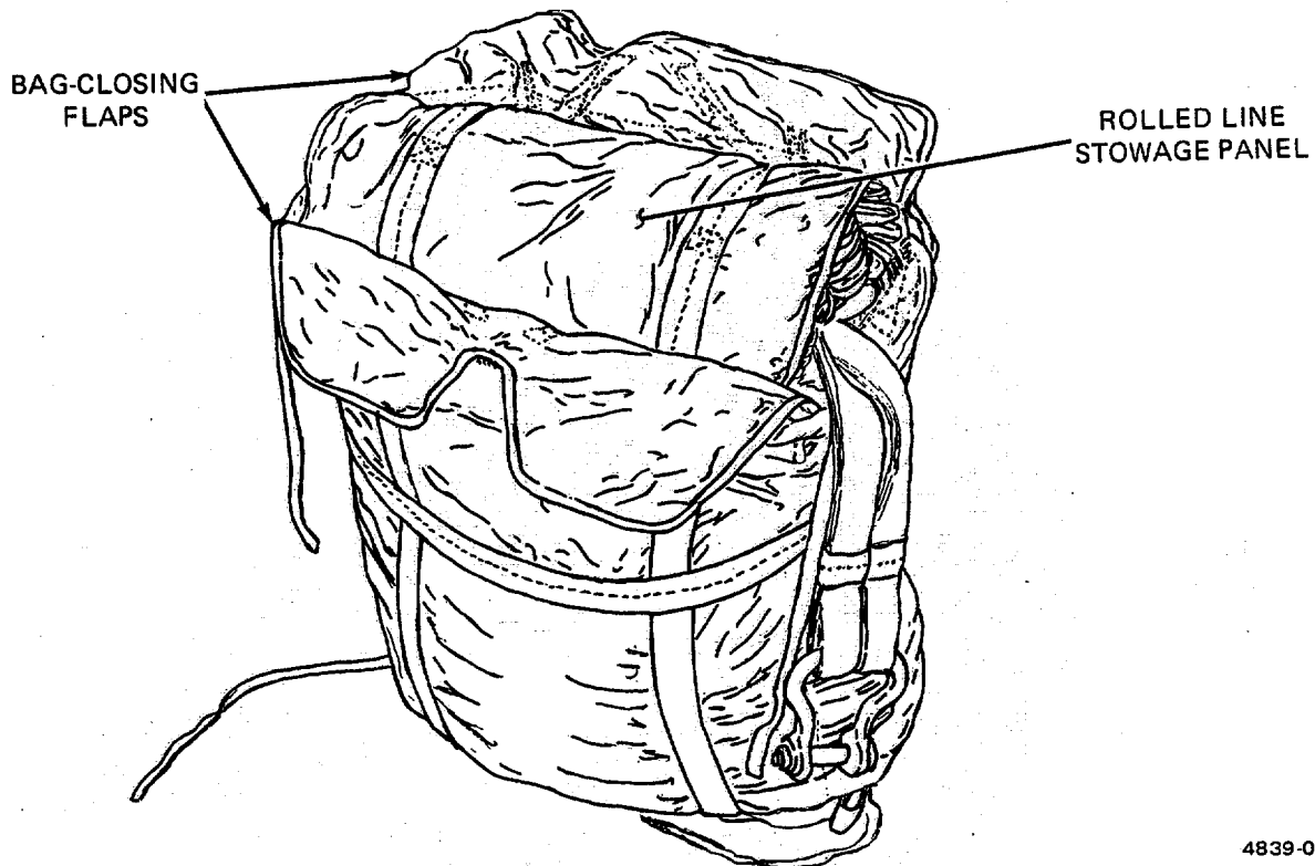
Figure 2-39. Suspension Line Stowage Panel Rolled and Inserted Into Bag Open End.
