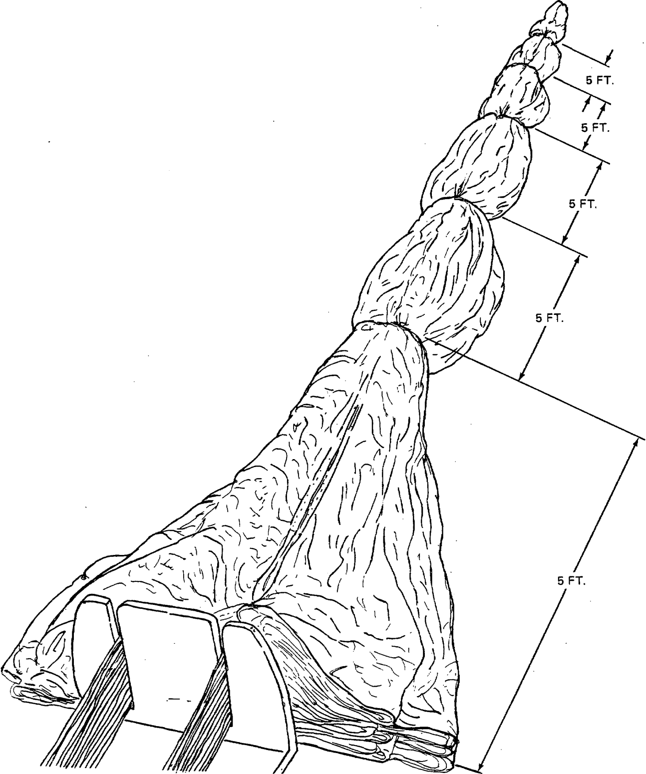
Figure 2-24. Canopy Ties Completed.
